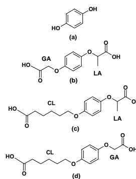
Figure 1. Novel unsymmetrical aromatic ether diacids where GA is glycolic acid, LA is Lactic acid and CL symbolizes Caprolactone unit
