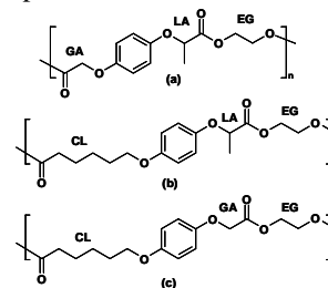
Figure 2. Absorbable polymers derived from novel unsymmetrical aromatic ether diacids where GA is glycolic acid, LA is Lactic acid and CL symbolizes caprolactone unit and EG stands for ethylene glycol unit.
