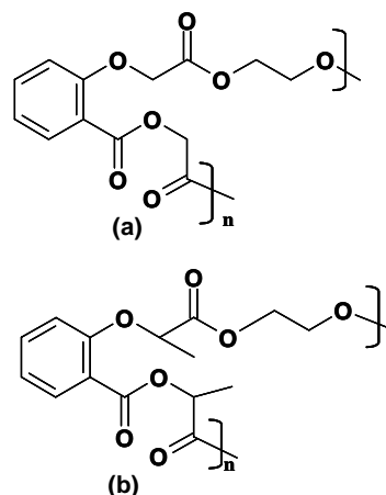
Figure 2 Absorbable polymers from functionalized Salicylic Acid
