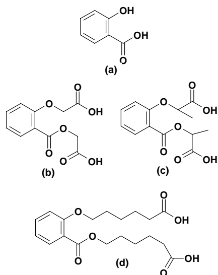
Figure 1. (a) Salicylic Acid (b) Glycolic acid functionalized Salicylic Acid (c) Lactic acid functionalized Salicylic Acid (d) Caprolactone functionalized Salicylic Acid
